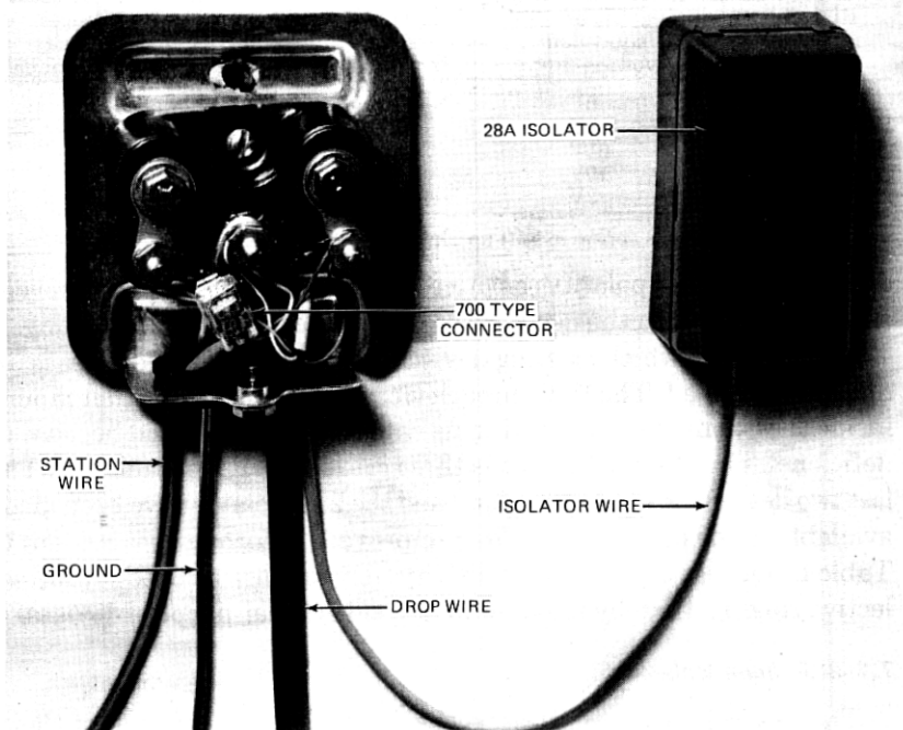
Fig. 22—28A ringer isolator mounted with station protector.
